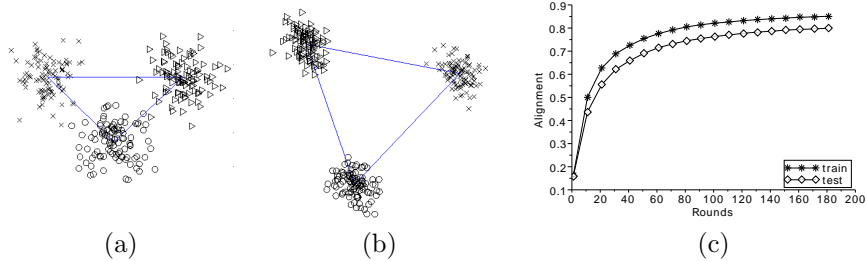
Fig. 1: Converge of the method to regular 2-simplex in 3 classes case after 2 steps(a) and 45 steps(b). Evolution of alignment for 10 classes(c)
